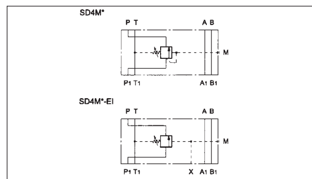
SIMBOLOS HIDRAULICOS HYDRAULIC SYMBOLS SYMBOLS HYDRAULIQUES
